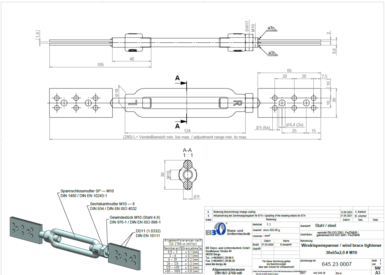
Figure A. 14 Wind brace tightener 30x65x2
